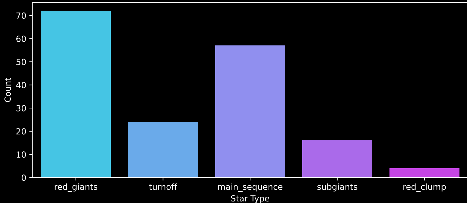
APOGEE DR17 Field: [060+56] Count plot of Star Type
