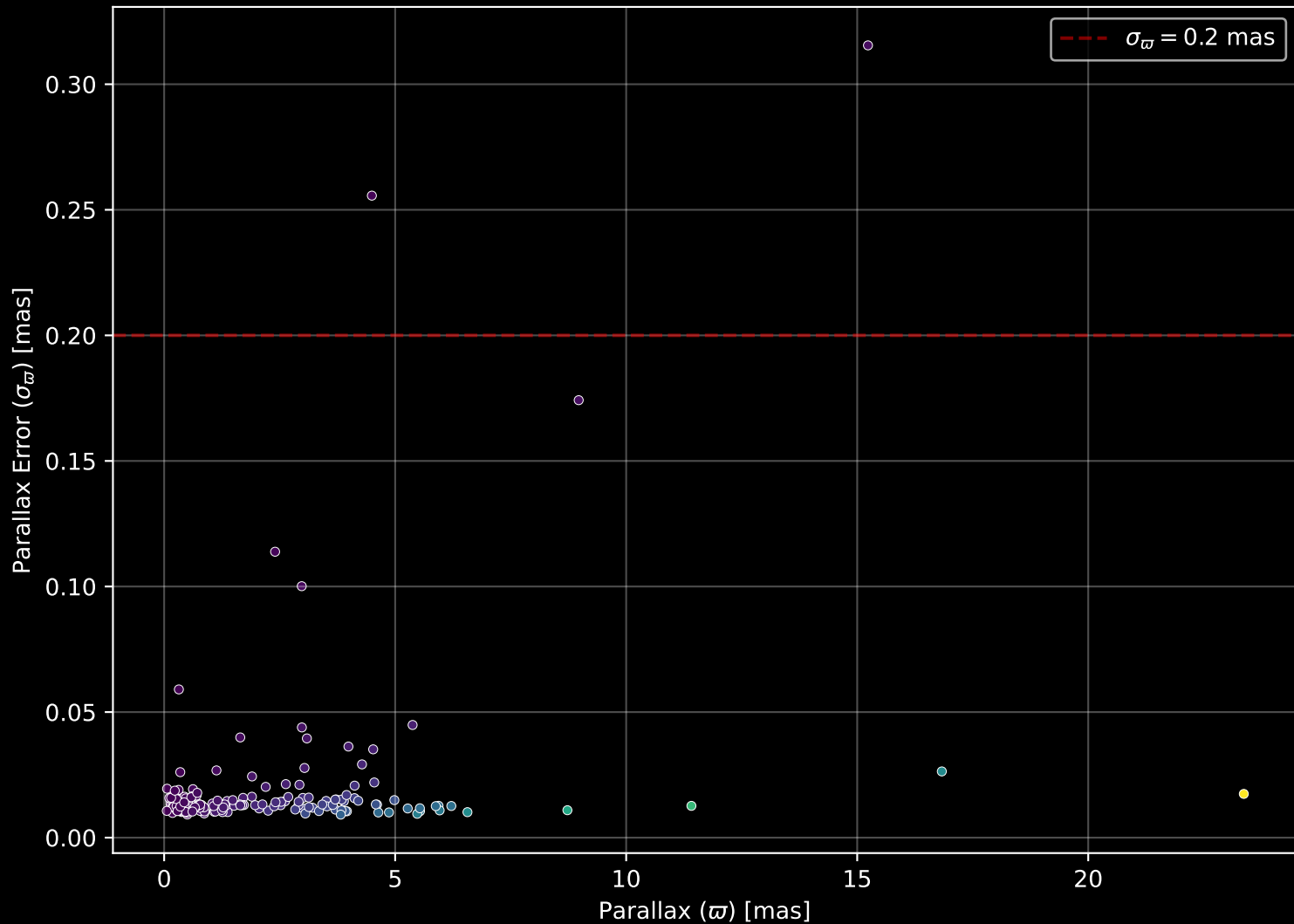
APOGEE DR17 Field: [060+56] Parallax Quality (n= 173)
