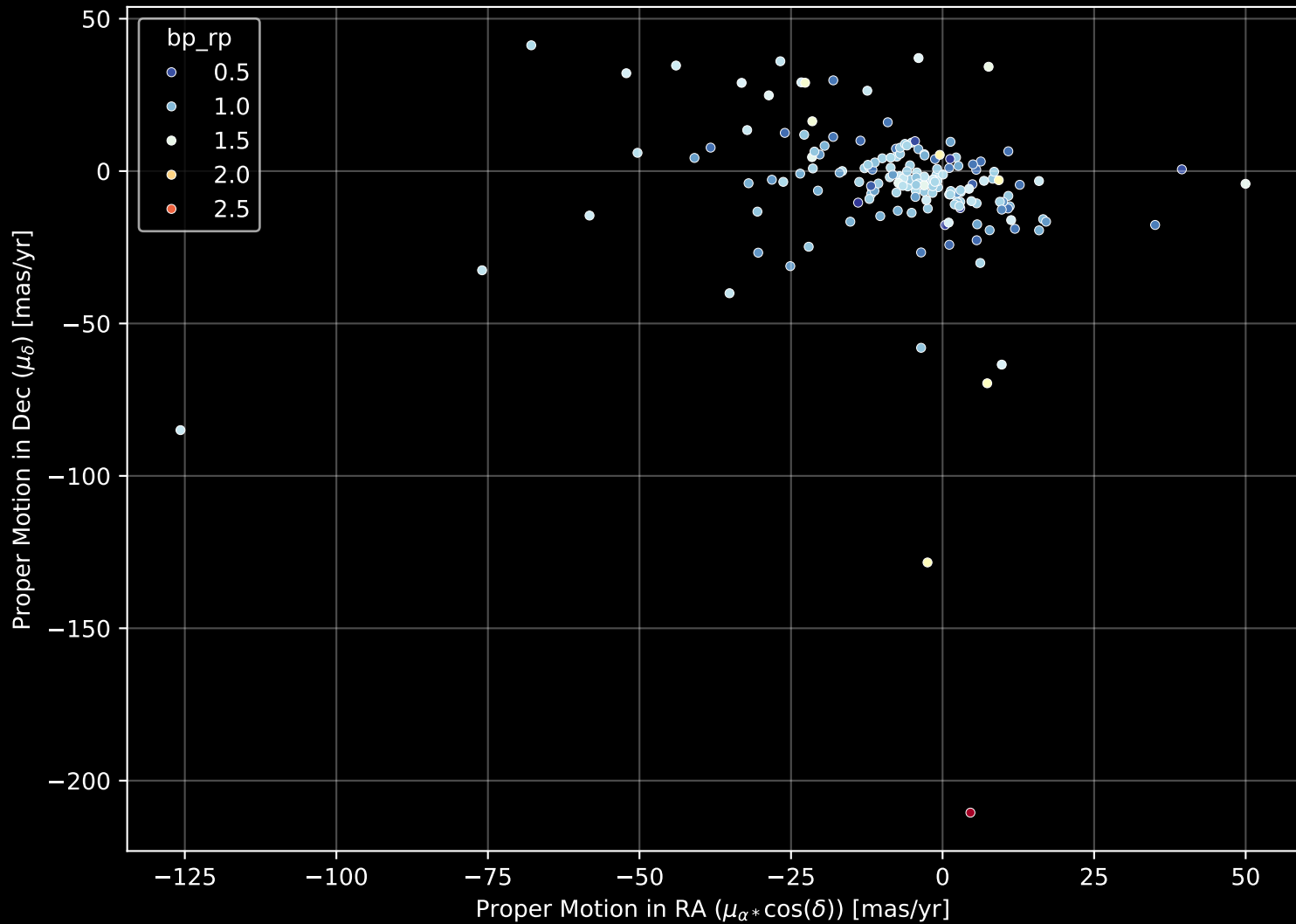
APOGEE DR17 Field: [060+56] Proper Motion Diagram (n= 173)
