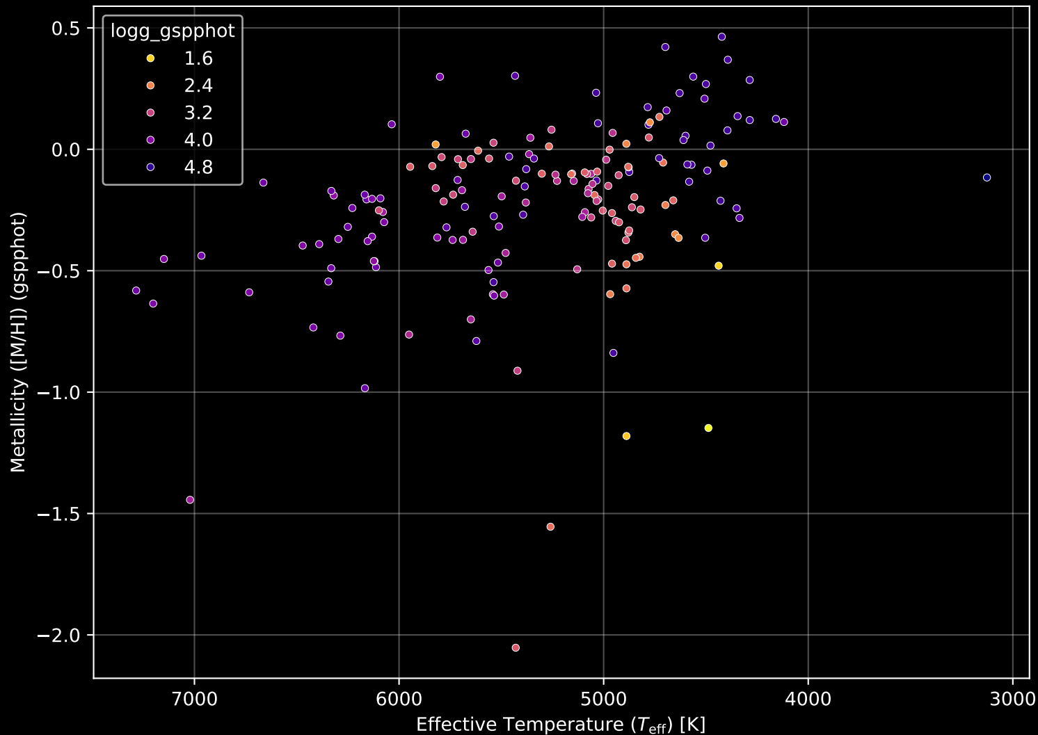
APOGEE DR17 Field: [060+56] Stellar Population Parameters (n= 173)
