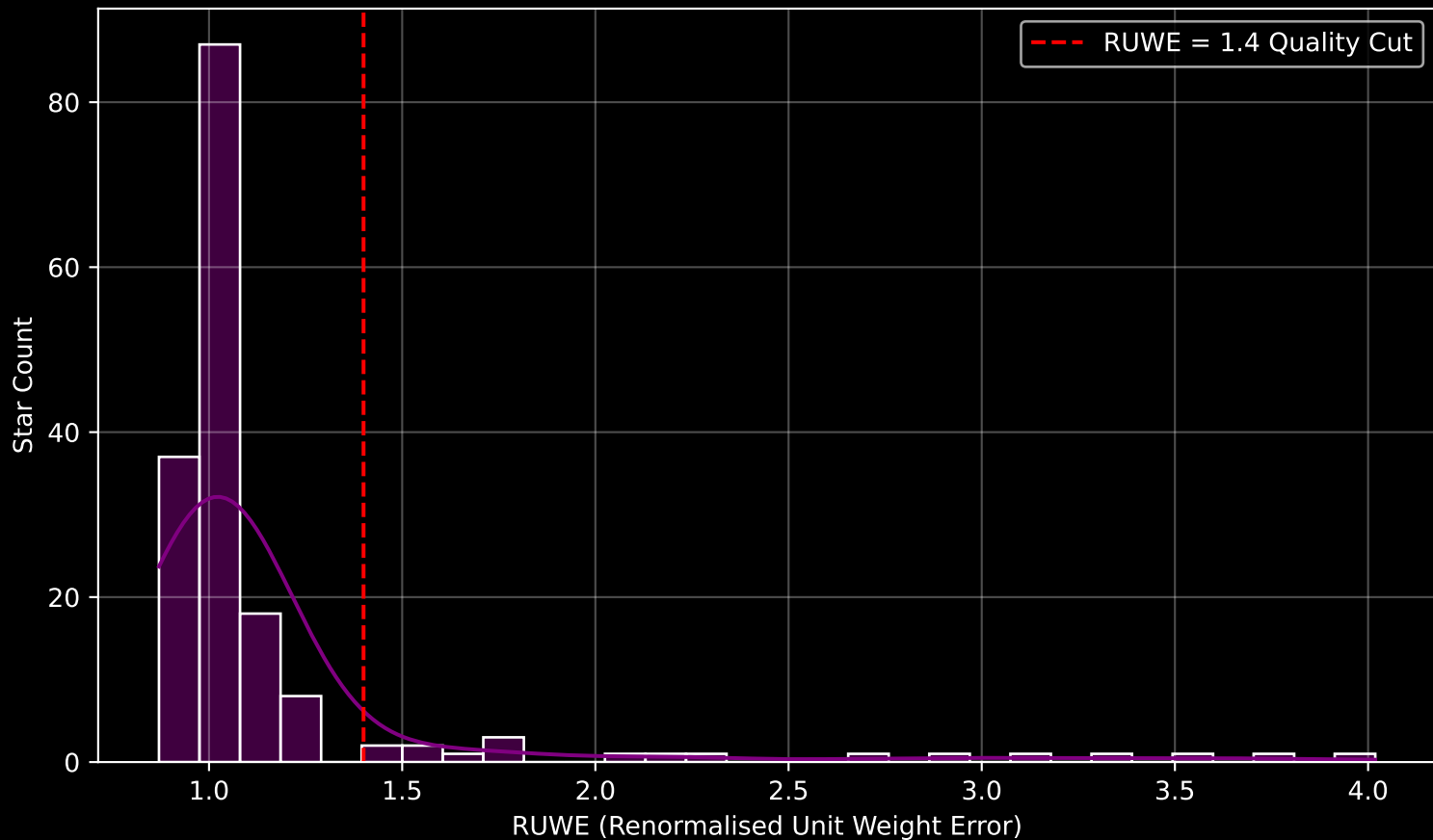
GAPOGEE DR17 Field [060+56] RUWE Distribution (n= 168)
