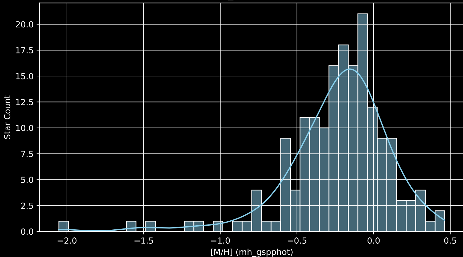
APOGEE DR17 Field: [060+56 [M/H] (mh_gspphot) (n= 173)
